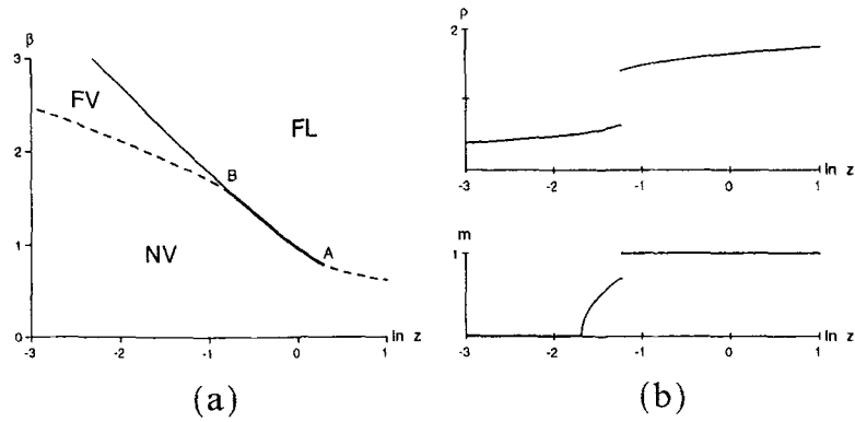
Fig. 2. The case J = 1 , g(\rho) = (\rho - 1)^4 . (a) Phase diagram. The bold and broken curves and the critical point A have the same meaning as in Fig. 1. In addition to the two phases NV and FL, there is an intermediate phase FV (ferromagnetic vapor); the solid line separating FV from FL indicates a first-order phase transition. Since the transition from NV to FV is second order, the critical point B is not a triple point. (b) Density and magnetization for \beta = 2 .
