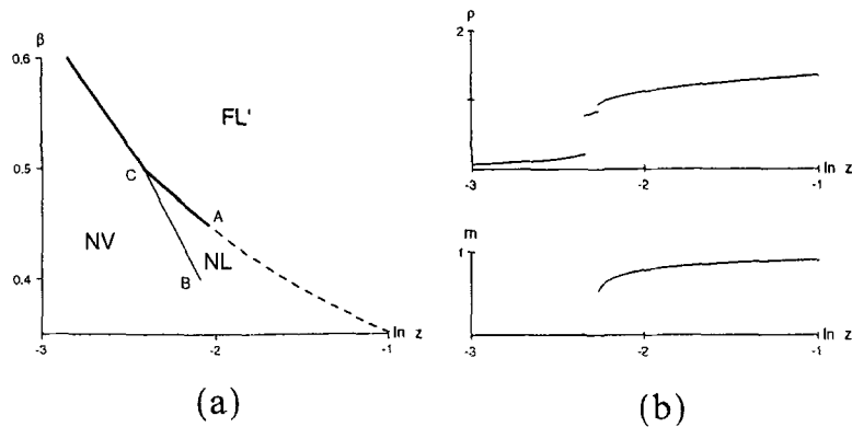
Fig. 3. The case J = 2.5 , g(\rho) = \rho^4 - 4\rho^2 . (a) Phase diagram. Bold and broken lines are as in Fig. 1. The solid line indicates a first-order vapor-liquid transition within the nonmagnetic region. The point C is a triple point of coexistence of three phases: nonmagnetic vapor (NV), nonmagnetic liquid (NL), and a ferromagnetic high-density phase which should probably also be interpreted as a liquid (FL'). B is the V-L critical point, and A the L-L' critical point. (b) Density and magnetization for \beta = 0.48 .
